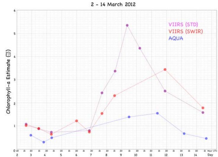
Comparisons of VIIRS and MODIS Chlorophyll Products for Early March at the Aeronet Site off the Los Angeles Coast.
